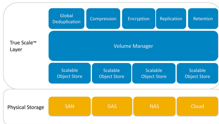
Figure 1. Architecture AppAssure True Scale
